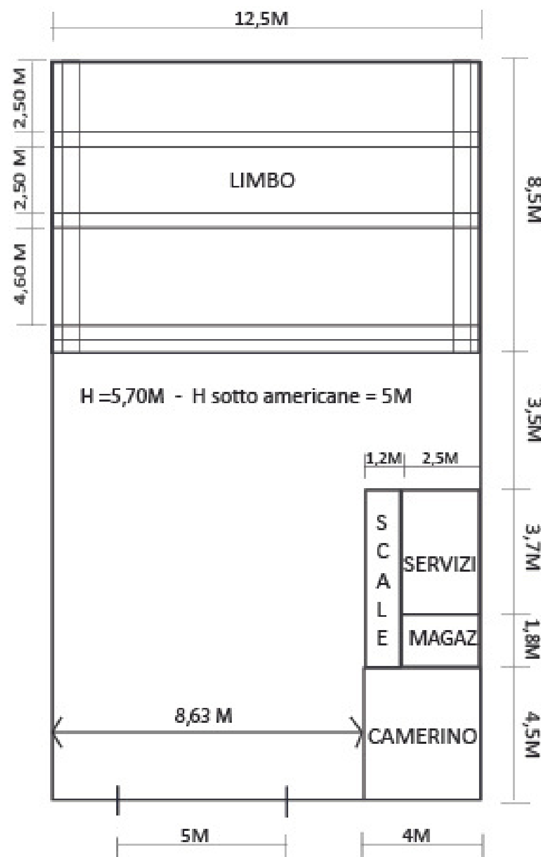
PIANO TERRA
